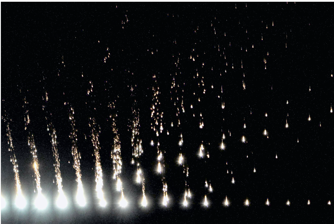
End of flight fragmentation of the November 18, 2012, fireball over the San Francisco Bay Area in California.
